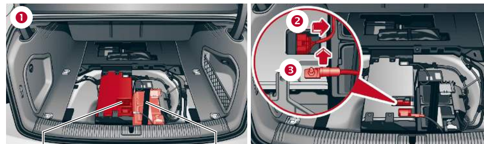
48-volt battery
