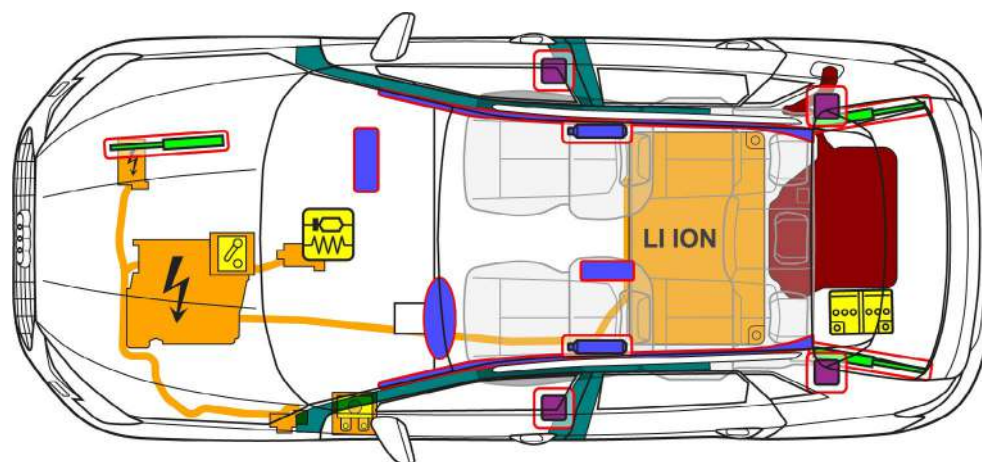
Rescue sheet for the Audi A3 TFSI e
