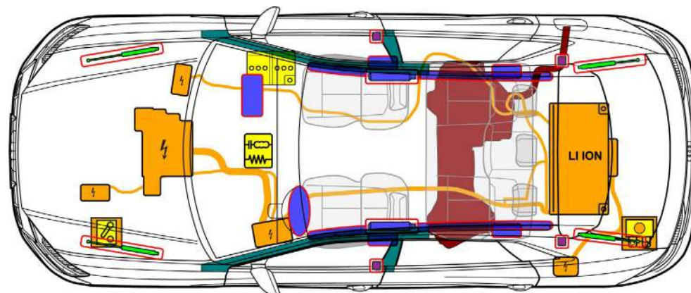
Rescue sheet for the Audi Q8 TFSI e
